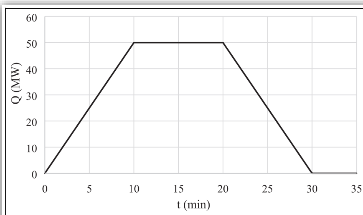
Figure I. The fire heat release rate with respect to time (CETU’s Guide to road tunnel safety documentation, 36 2003).
