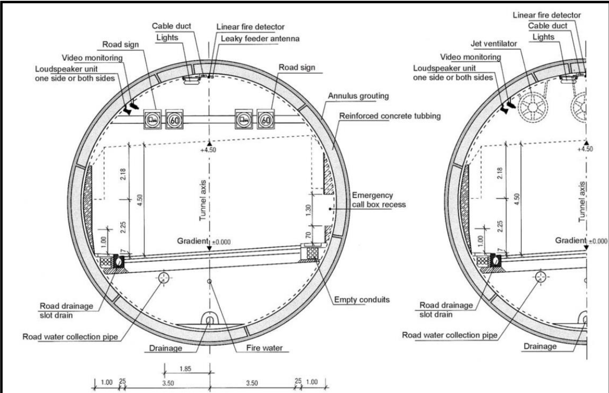
Figure 5: Equipment example circular cross section – tubing – depiction of the technical possibilities
