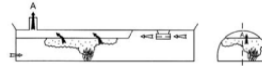
Figure 8: Longitudinal ventilation and smoke extraction for the event of a fire
