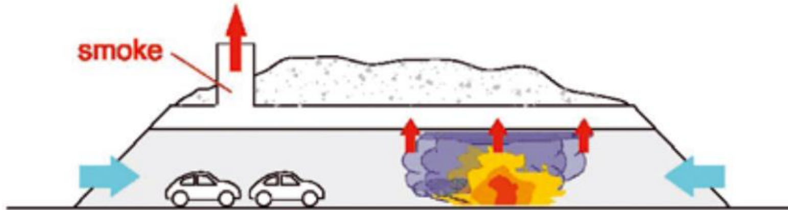
FIGURE 3 - SEMI-TRANSVERSE VENTILATION: DURING NORMAL OPERATING CONDITIONS; FRESH AIR INJECTION
