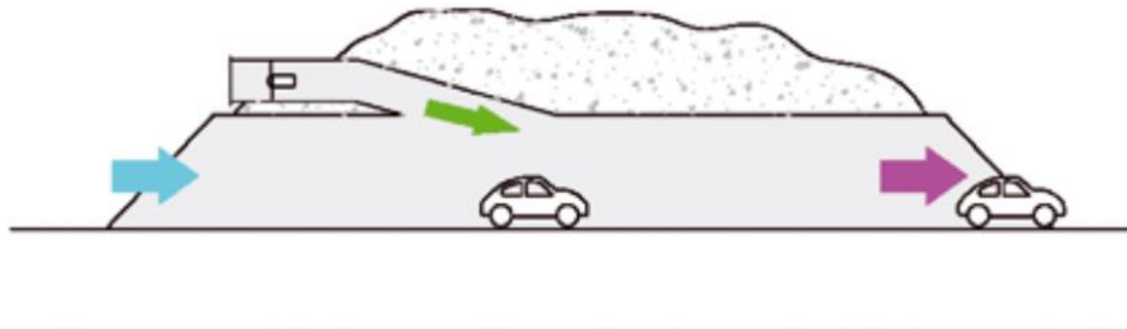
FIGURE 2 - LONGITUDINAL VENTILATION WITH SACCARDO NOZZLE
