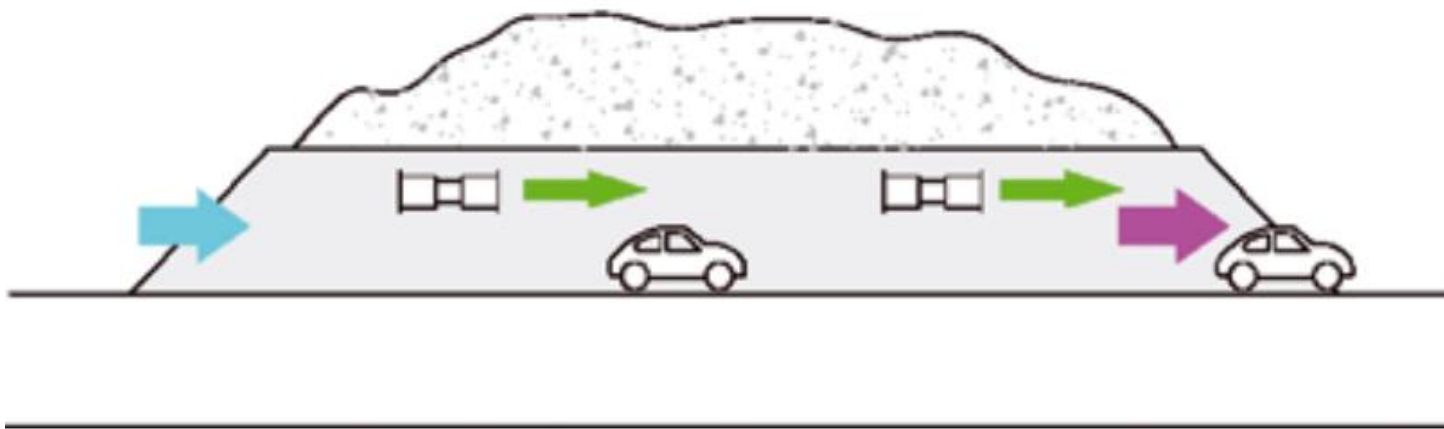
FIGURE 1 - LONGITUDINAL VENTILATION WITH JET FANS
